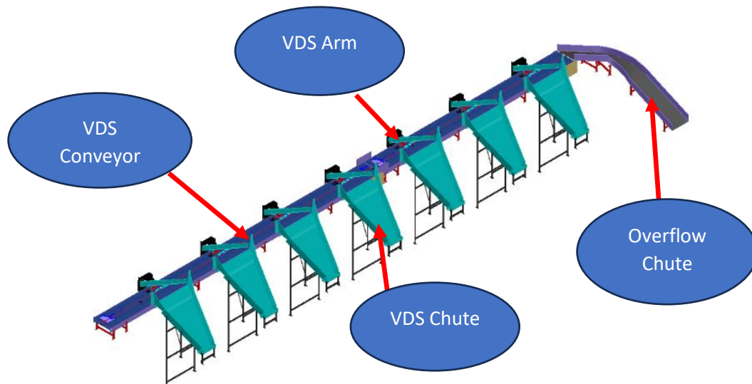
Arm Based Volume Distribution System
